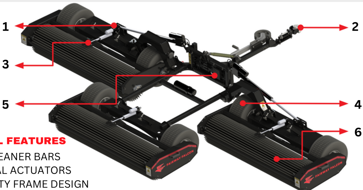
4. TURF TIRES 18" TURF TIRES USED TO REDUCE COMPACTION
